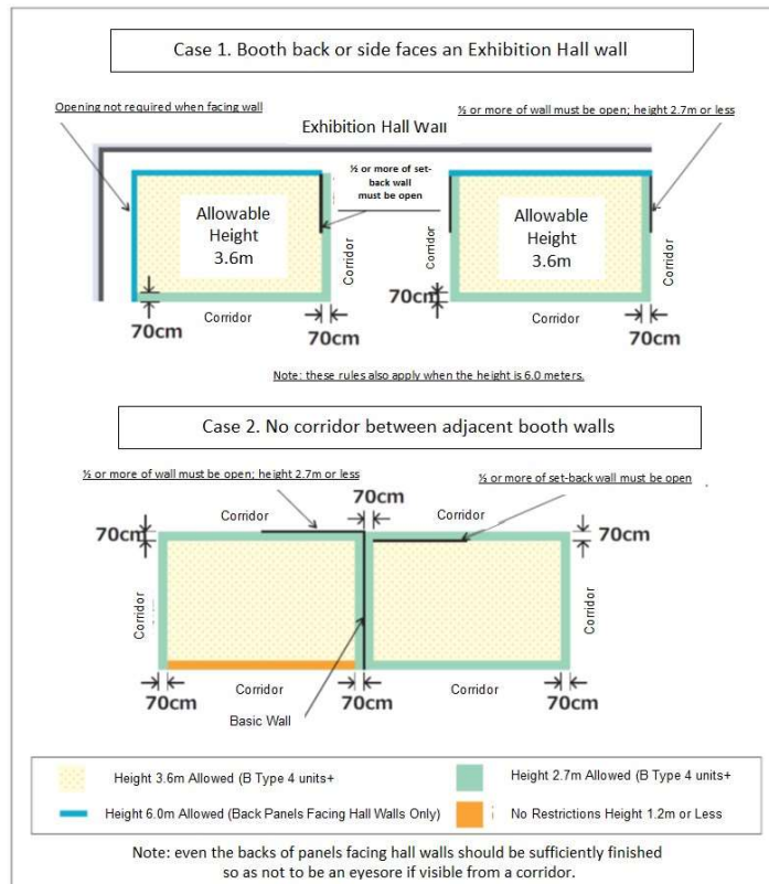
Figure 2. Limitations on Booth Height and Required Openings
